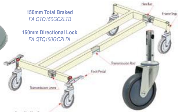
Central Locking Castor
